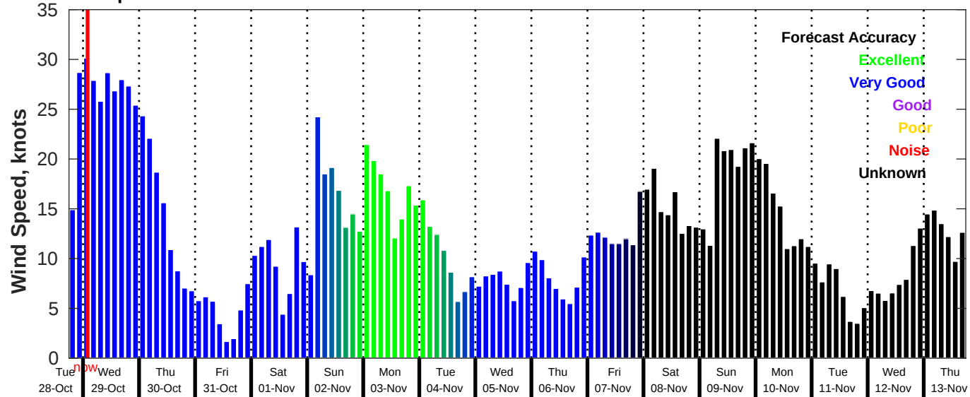
GFS Wind Speed Forecast for NDBC 42035 from 28-Oct-2025 18:00:00 to 13-Nov-2025 18:00:00
