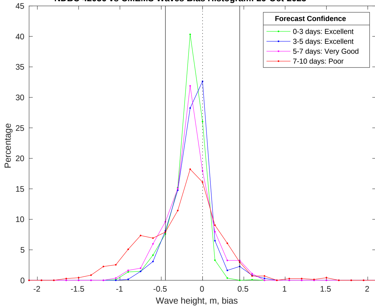
NDBC 42036 vs CMEMS Waves Bias Histogram: 29-Oct-2025
