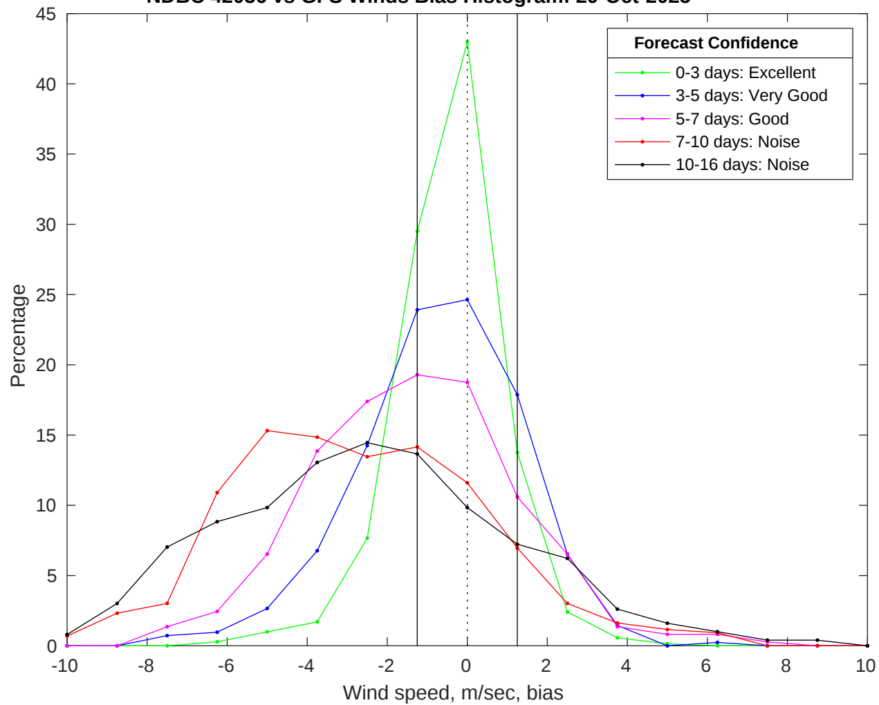
NDBC 42036 vs GFS Winds Bias Histogram: 29-Oct-2025
