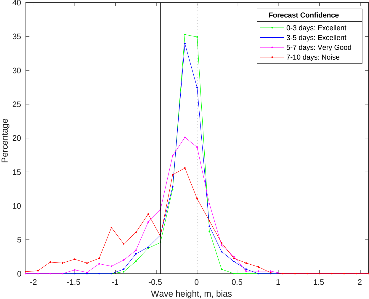
NDBC 42040 vs CMEMS Waves Bias Histogram: 29-Oct-2025
