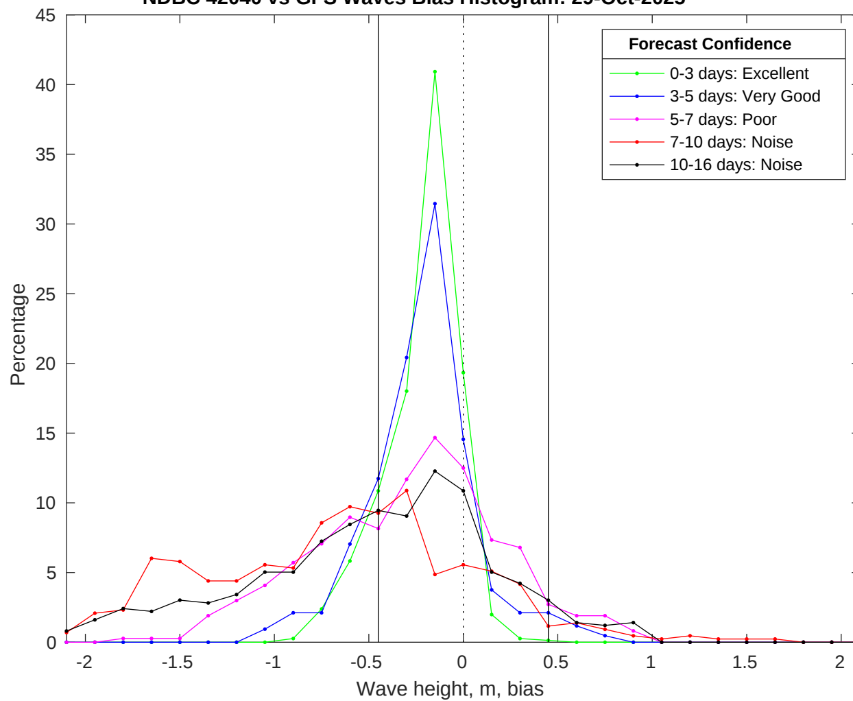
NDBC 42040 vs GFS Waves Bias Histogram: 29-Oct-2025
