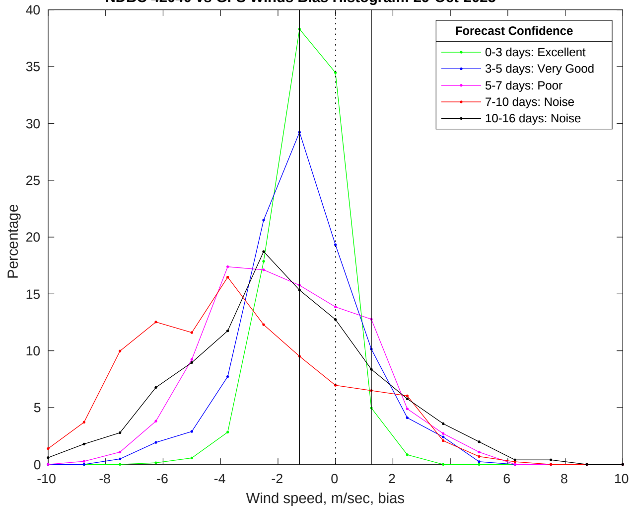
NDBC 42040 vs GFS Winds Bias Histogram: 29-Oct-2025
