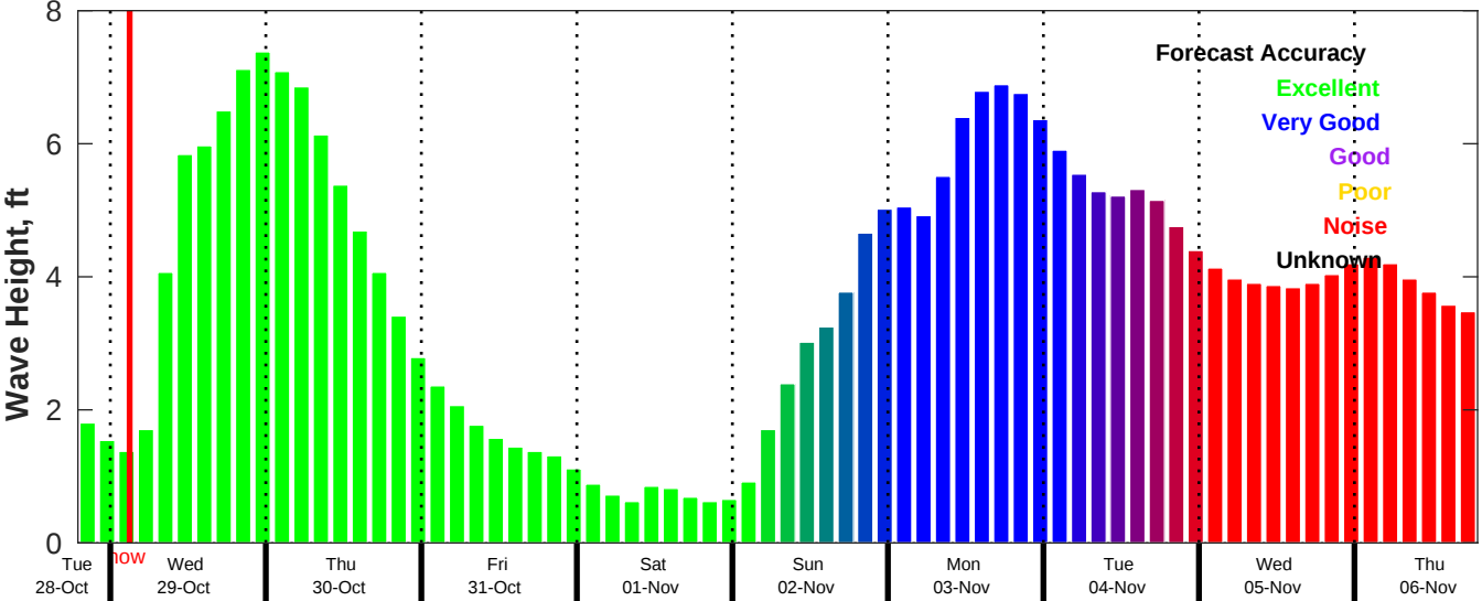
CMEMS Wave Forecast for NDBC 42040 from 28-Oct-2025 19:00:00 to 06-Nov-2025 19:00:00
