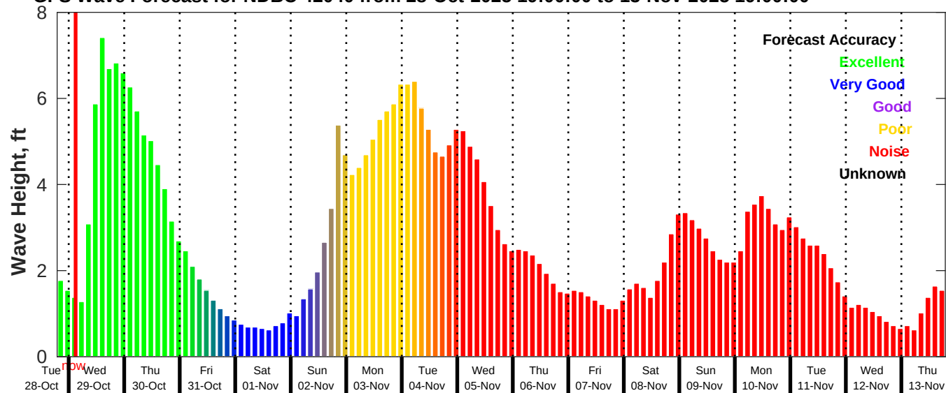
GFS Wave Forecast for NDBC 42040 from 28-Oct-2025 19:00:00 to 13-Nov-2025 19:00:00
