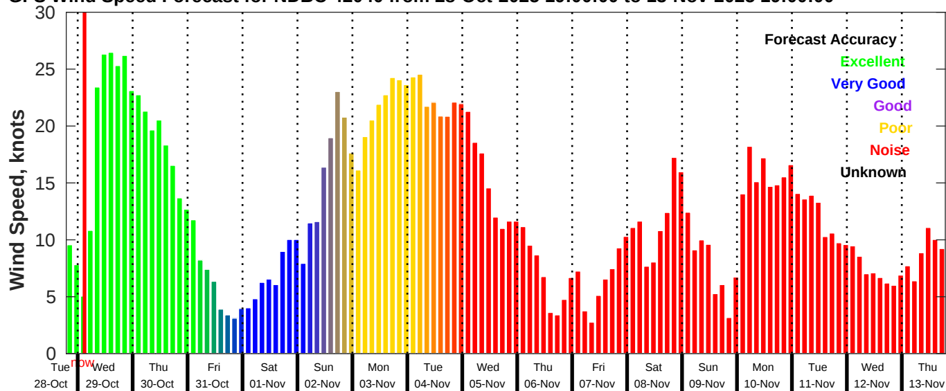
GFS Wind Speed Forecast for NDBC 42040 from 28-Oct-2025 19:00:00 to 13-Nov-2025 19:00:00
