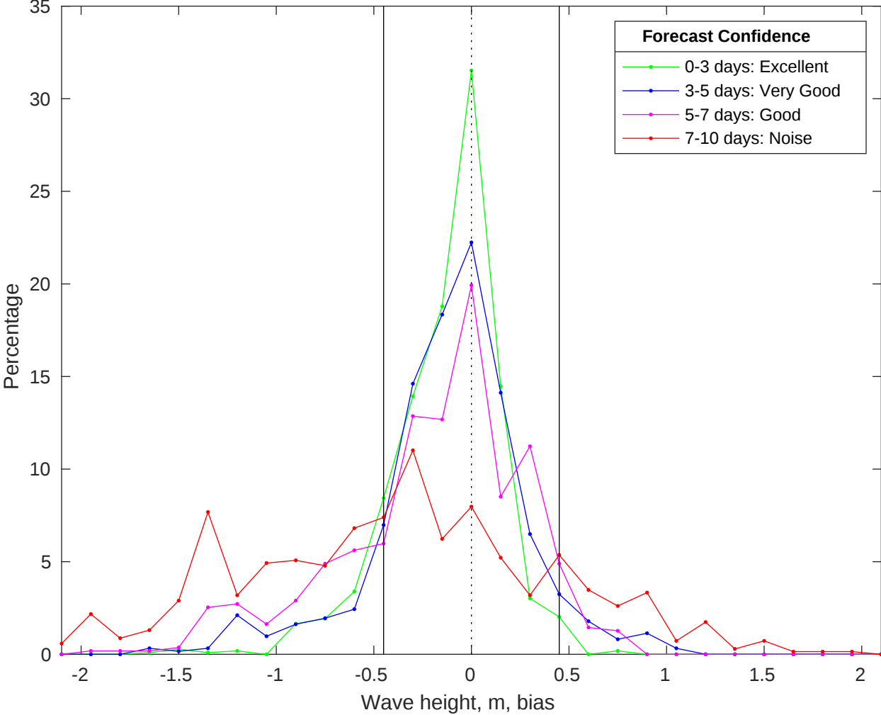
NDBC 44008 vs CMEMS Waves Bias Histogram: 29-Oct-2025
