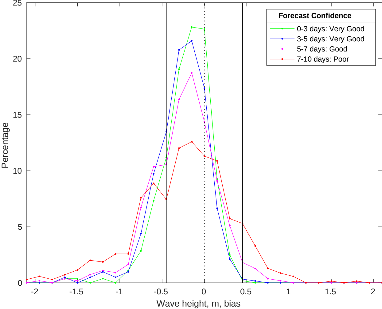
NDBC 46011 vs CMEMS Waves Bias Histogram: 29-Oct-2025
