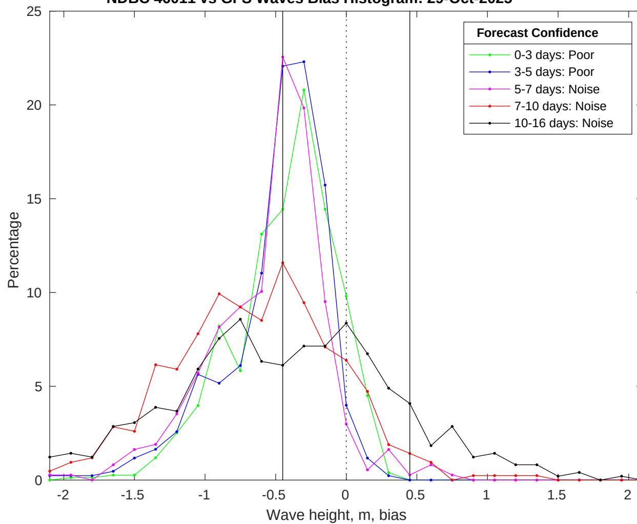
NDBC 46011 vs GFS Waves Bias Histogram: 29-Oct-2025
