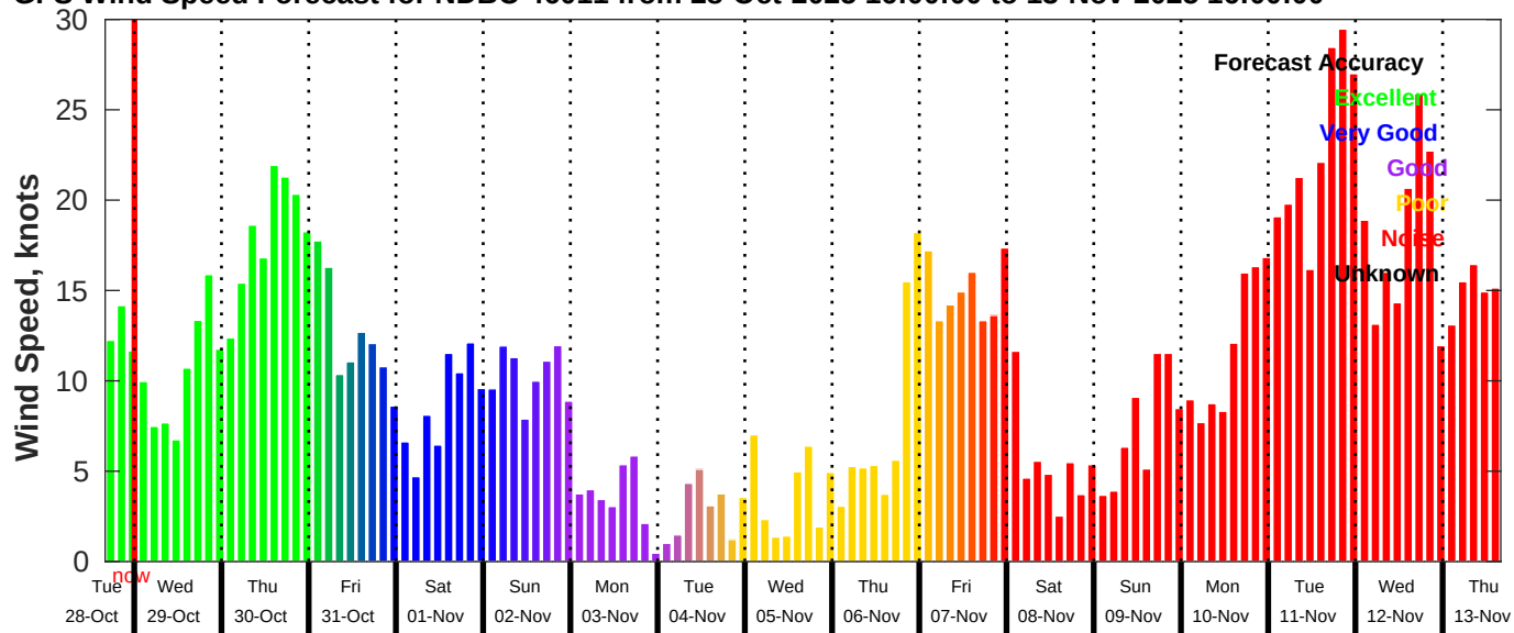
GFS Wind Speed Forecast for NDBC 46011 from 28-Oct-2025 16:00:00 to 13-Nov-2025 16:00:00
