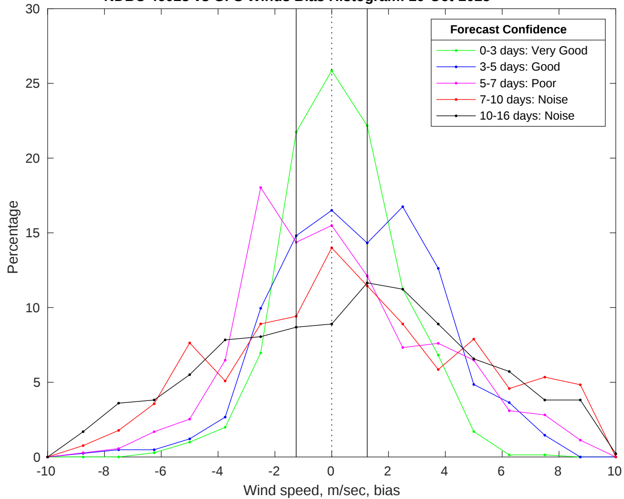
NDBC 46028 vs GFS Winds Bias Histogram: 29-Oct-2025
