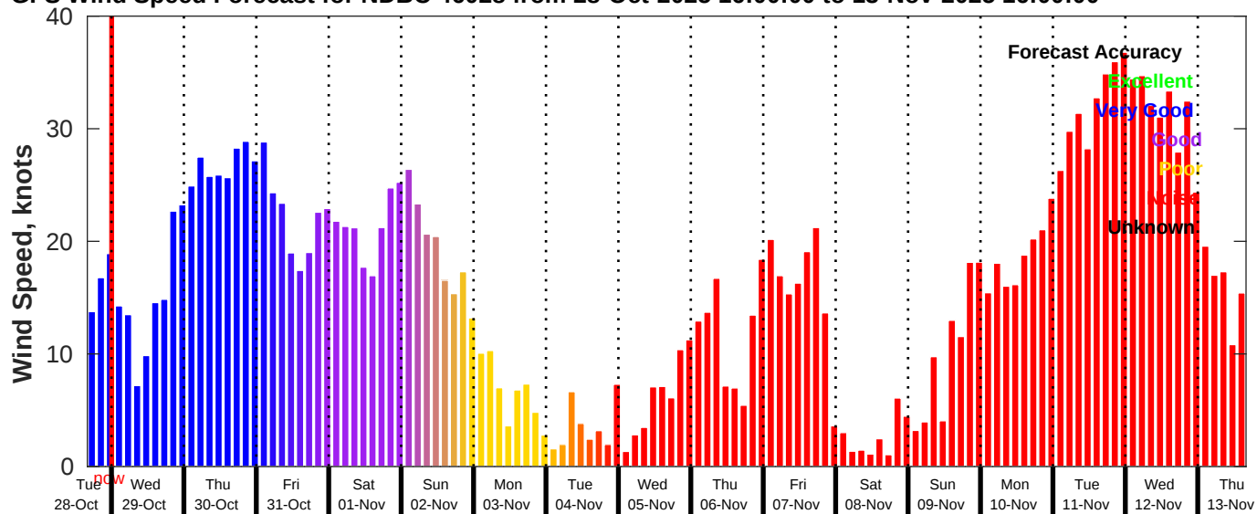
GFS Wind Speed Forecast for NDBC 46028 from 28-Oct-2025 16:00:00 to 13-Nov-2025 16:00:00
