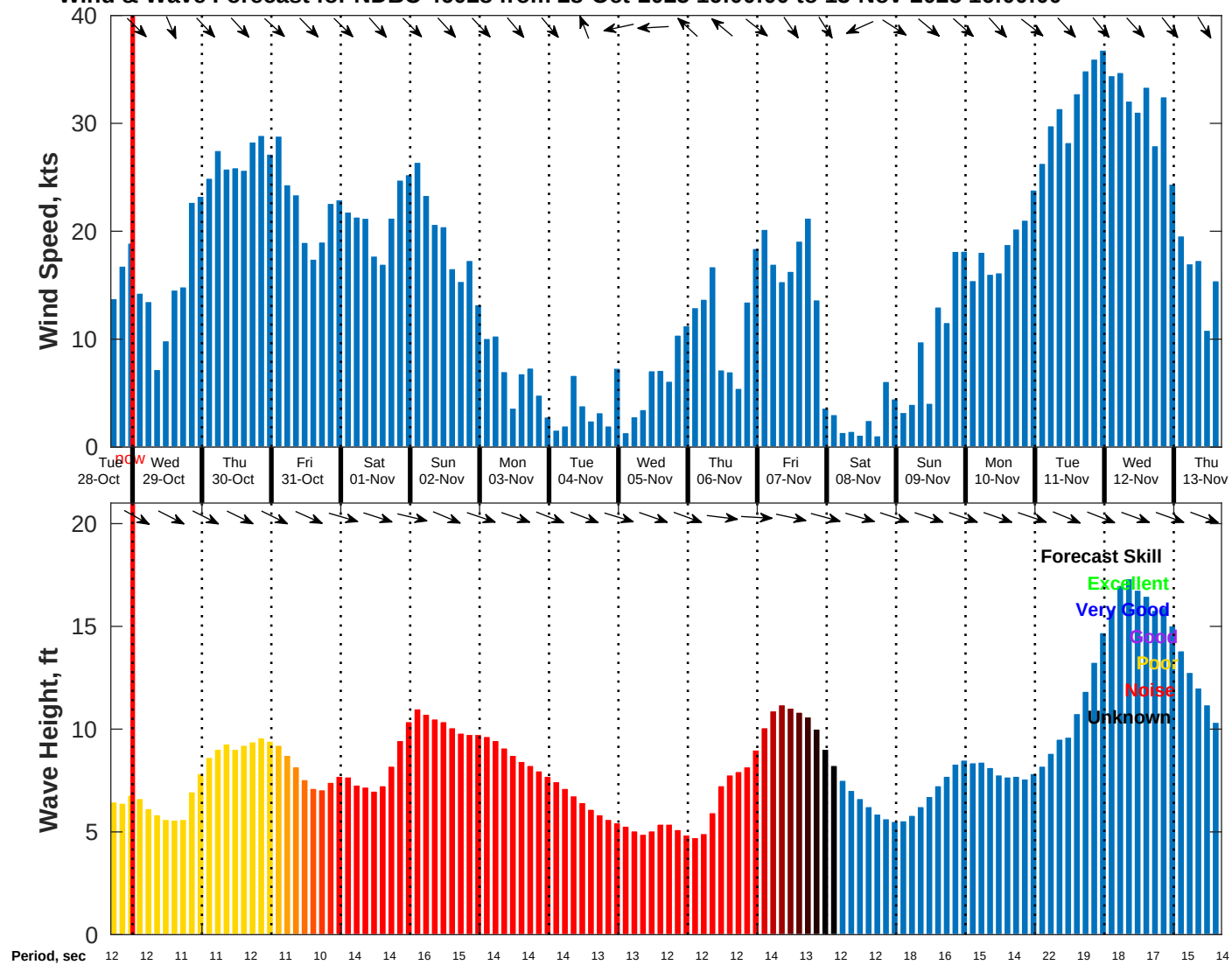
Wind & Wave Forecast for NDBC 46028 from 28-Oct-2025 16:00:00 to 13-Nov-2025 16:00:00
