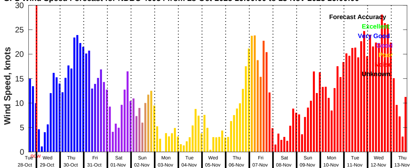
GFS Wind Speed Forecast for NDBC 46054 from 28-Oct-2025 16:00:00 to 13-Nov-2025 16:00:00
