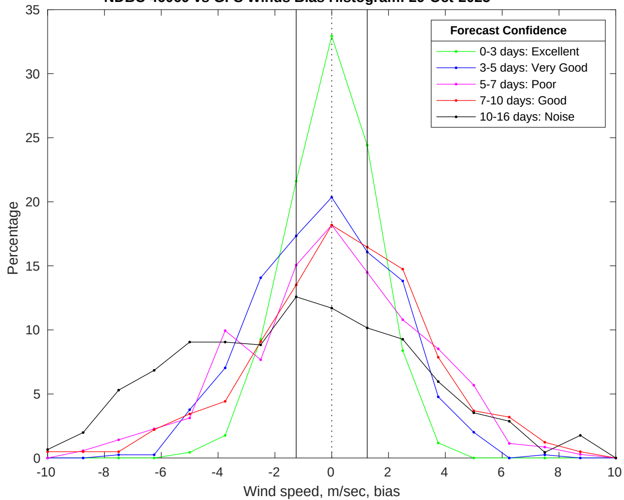
NDBC 46069 vs GFS Winds Bias Histogram: 29-Oct-2025
