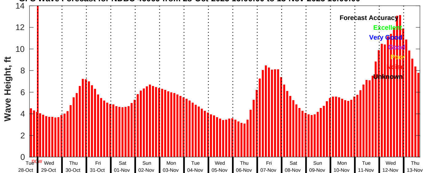
GFS Wave Forecast for NDBC 46069 from 28-Oct-2025 16:00:00 to 13-Nov-2025 16:00:00
