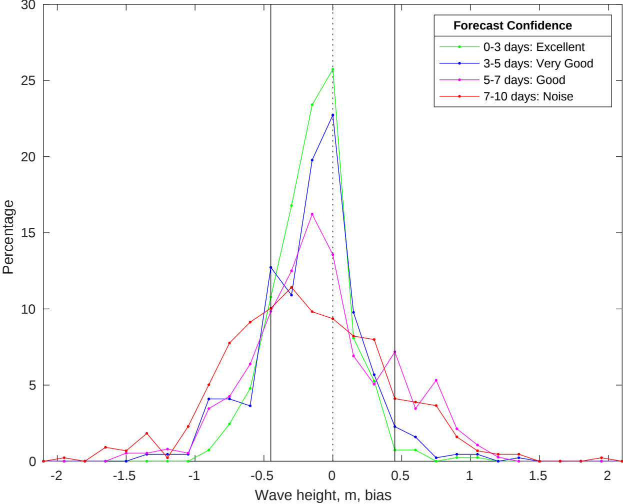
NDBC 46259 vs CMEMS Waves Bias Histogram: 29-Oct-2025
