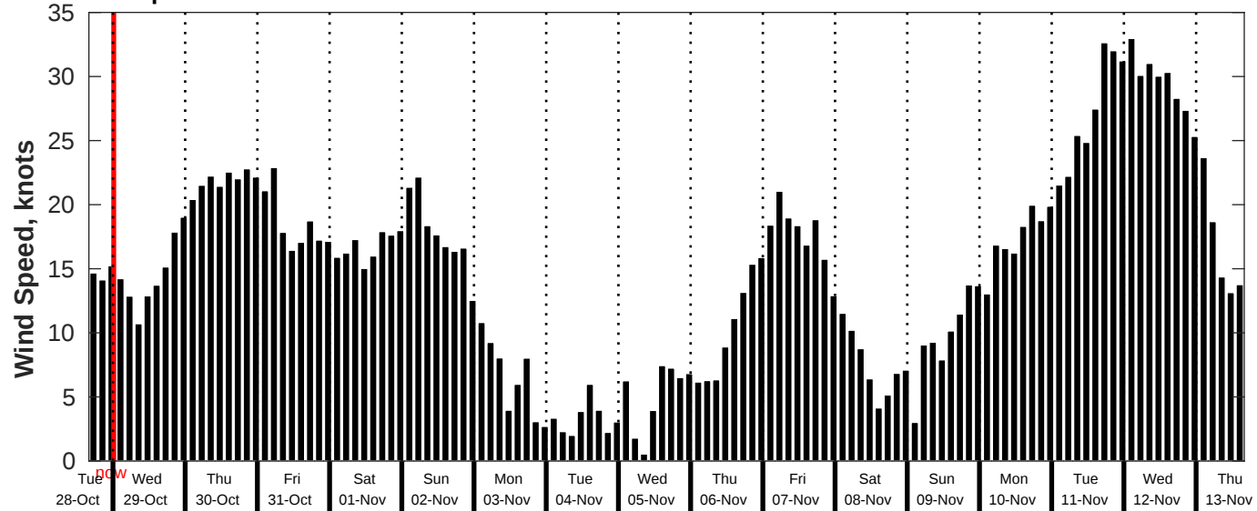
GFS Wind Speed Forecast for NDBC 46259 from 28-Oct-2025 16:00:00 to 13-Nov-2025 16:00:00
