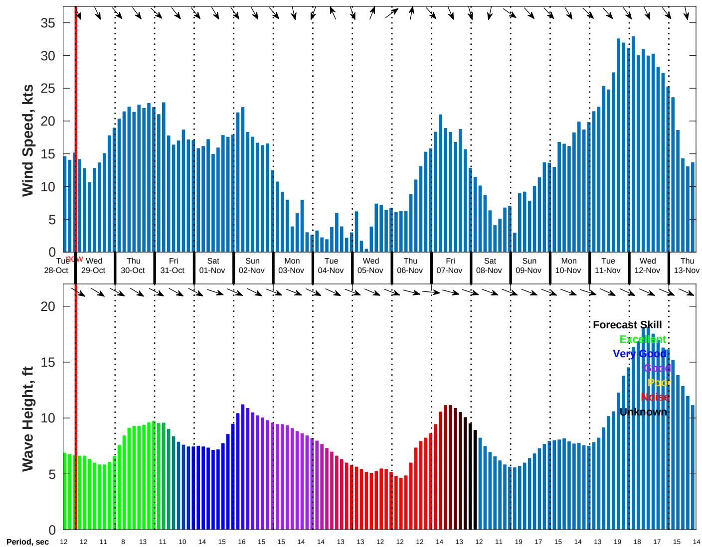
Wind & Wave Forecast for NDBC 46259 from 28-Oct-2025 16:00:00 to 13-Nov-2025 16:00:00
