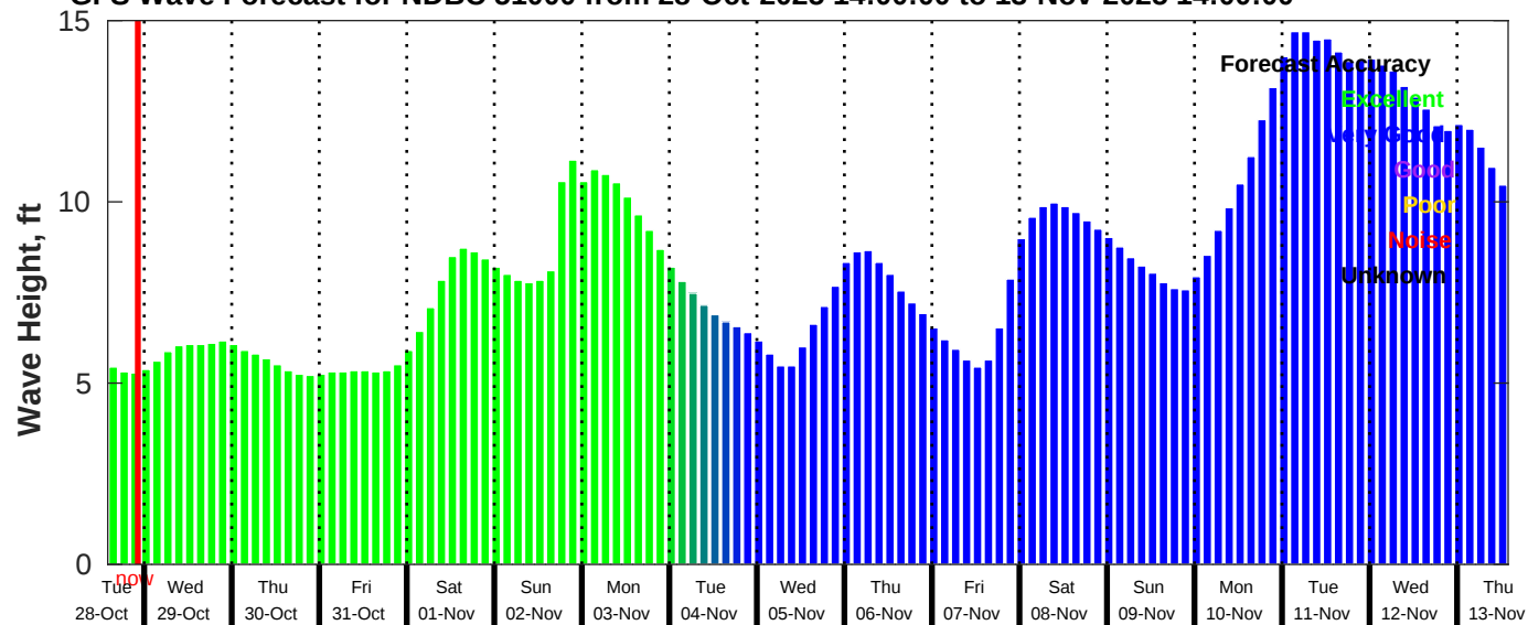
GFS Wave Forecast for NDBC 51000 from 28-Oct-2025 14:00:00 to 13-Nov-2025 14:00:00
