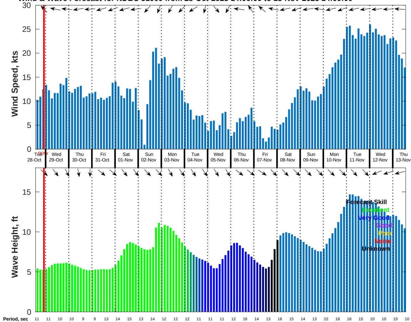
Wind & Wave Forecast for NDBC 51000 from 28-Oct-2025 14:00:00 to 13-Nov-2025 14:00:00
