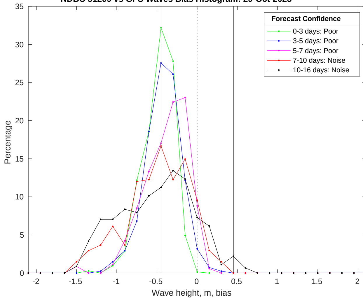
NDBC 51209 vs GFS Waves Bias Histogram: 29-Oct-2025
