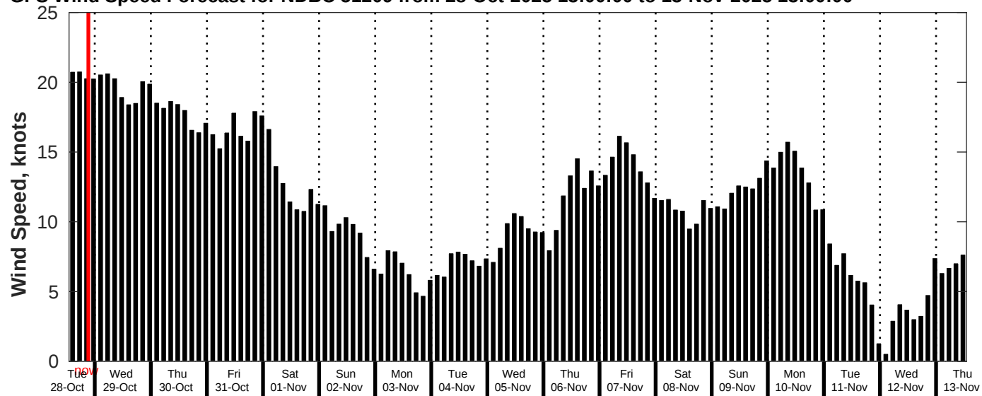
GFS Wind Speed Forecast for NDBC 51209 from 28-Oct-2025 13:00:00 to 13-Nov-2025 13:00:00
