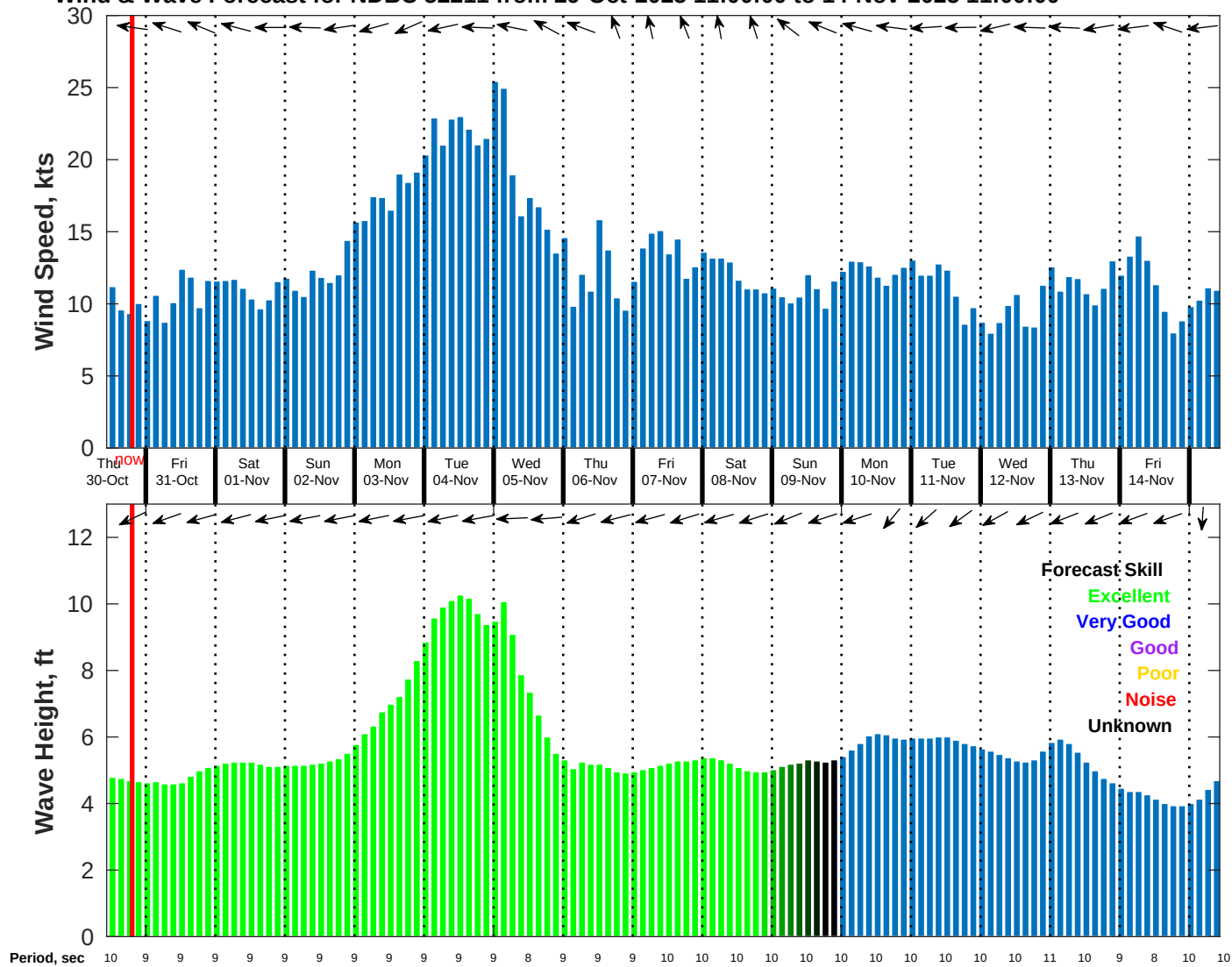
Wind & Wave Forecast for NDBC 52211 from 29-Oct-2025 11:00:00 to 14-Nov-2025 11:00:00
