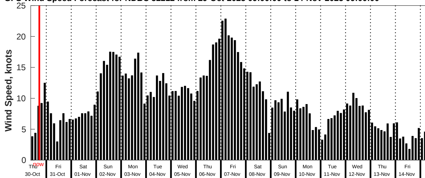
GFS Wind Speed Forecast for NDBC 52212 from 29-Oct-2025 09:00:00 to 14-Nov-2025 09:00:00
