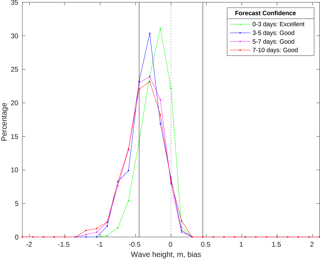
NDBC 52213 vs CMEMS Waves Bias Histogram: 29-Oct-2025
