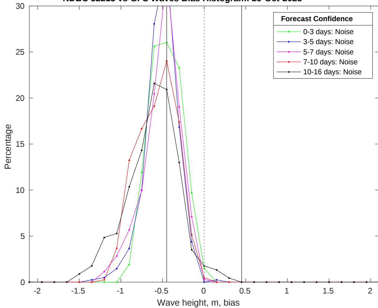
NDBC 52213 vs GFS Waves Bias Histogram: 29-Oct-2025
