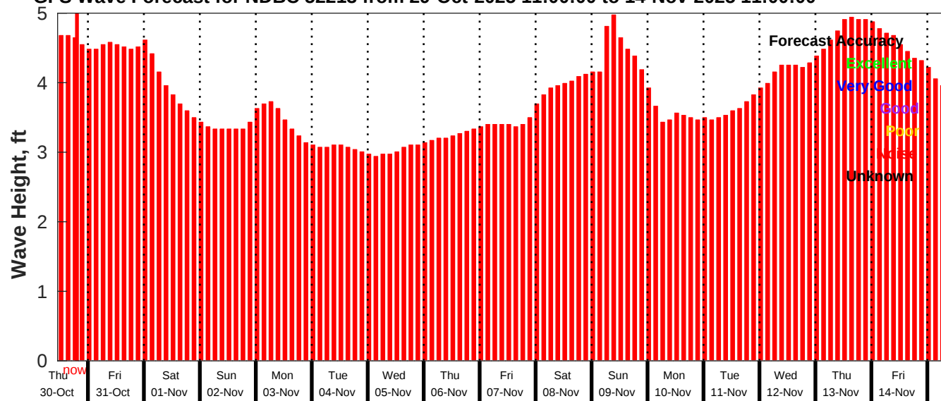
GFS Wave Forecast for NDBC 52213 from 29-Oct-2025 11:00:00 to 14-Nov-2025 11:00:00
