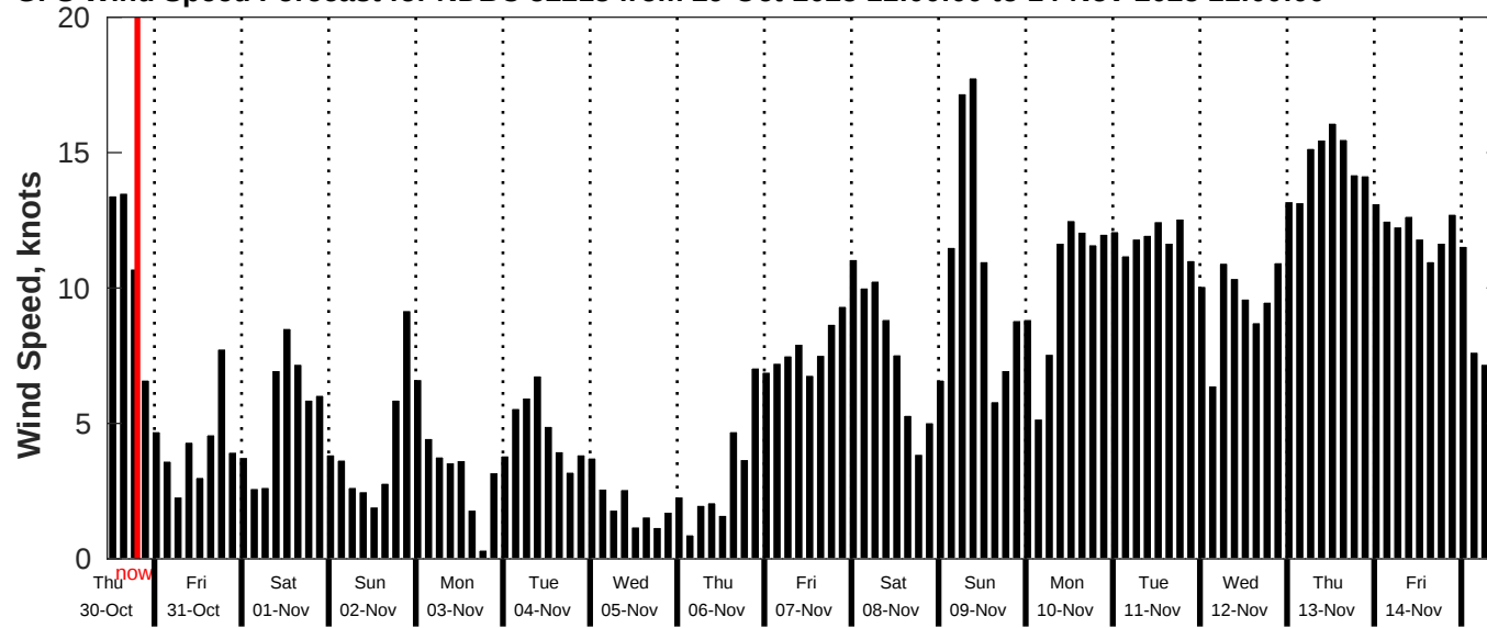
GFS Wind Speed Forecast for NDBC 52213 from 29-Oct-2025 11:00:00 to 14-Nov-2025 11:00:00
