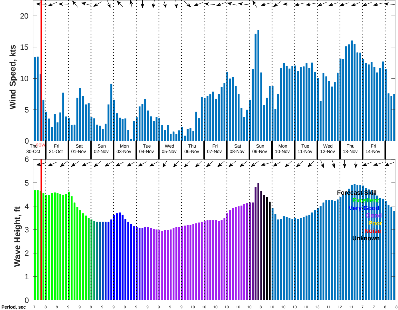
Wind & Wave Forecast for NDBC 52213 from 29-Oct-2025 11:00:00 to 14-Nov-2025 11:00:00
