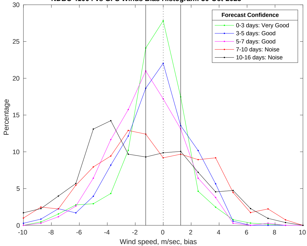
NDBC 41004 vs GFS Winds Bias Histogram: 30-Oct-2025
