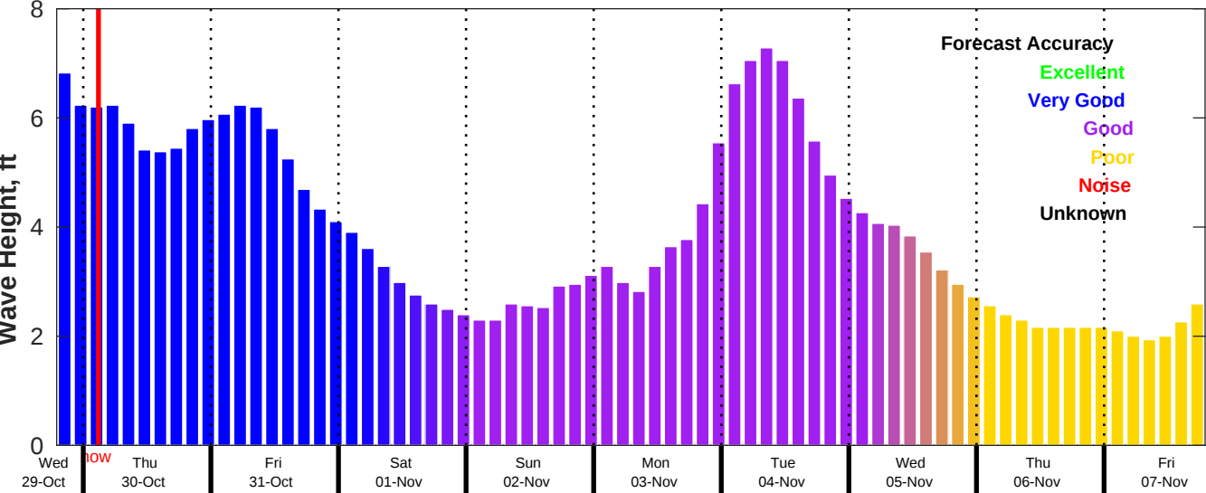
CMEMS Wave Forecast for NDBC 41004 from 29-Oct-2025 19:00:00 to 07-Nov-2025 19:00:00
