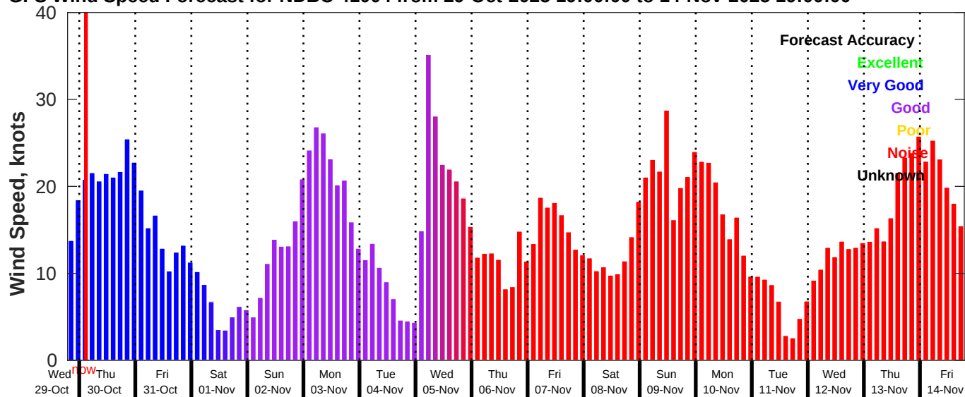
GFS Wind Speed Forecast for NDBC 41004 from 29-Oct-2025 19:00:00 to 14-Nov-2025 19:00:00
