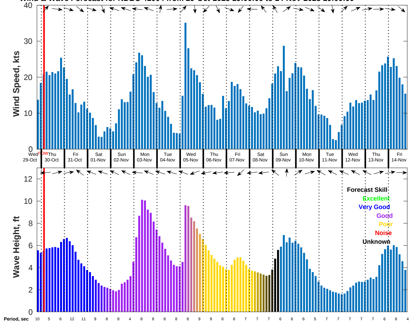
Wind & Wave Forecast for NDBC 41004 from 29-Oct-2025 19:00:00 to 14-Nov-2025 19:00:00
