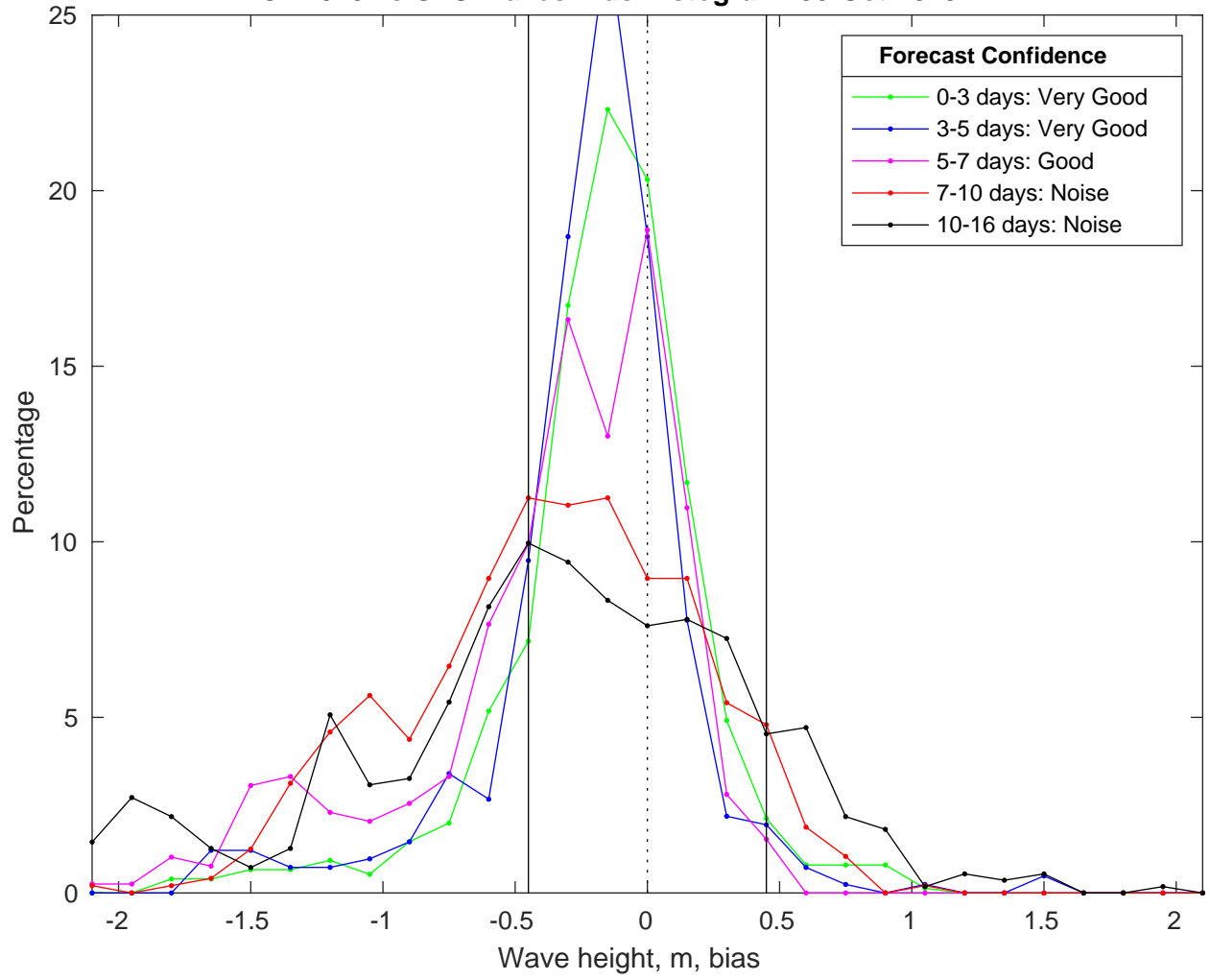
NDBC 41013 vs GFS Waves Bias Histogram: 30-Oct-2025
