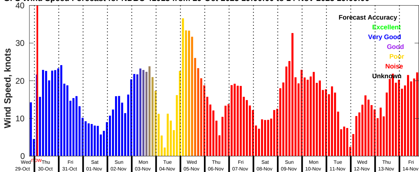
GFS Wind Speed Forecast for NDBC 41013 from 29-Oct-2025 19:00:00 to 14-Nov-2025 19:00:00
