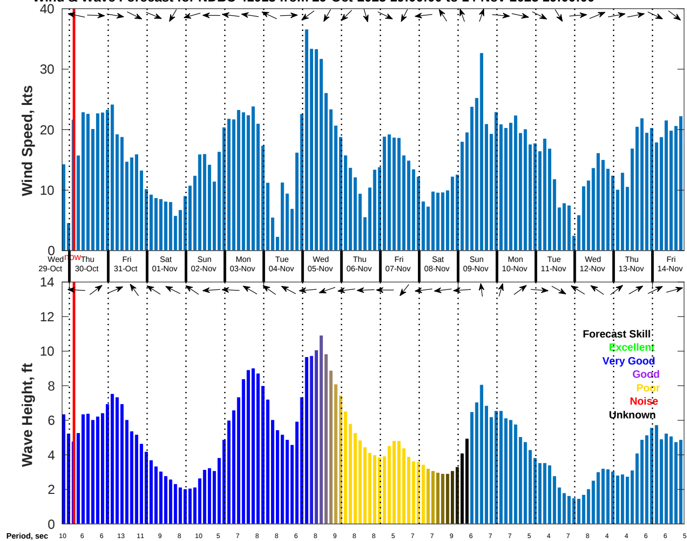
Wind & Wave Forecast for NDBC 41013 from 29-Oct-2025 19:00:00 to 14-Nov-2025 19:00:00
