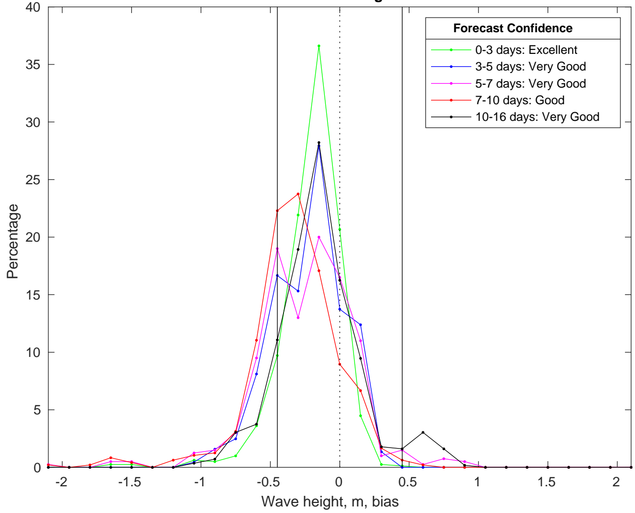
NDBC 41040 vs GFS Waves Bias Histogram: 30-Oct-2025
