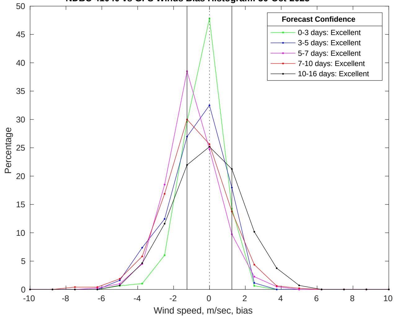
NDBC 41040 vs GFS Winds Bias Histogram: 30-Oct-2025
