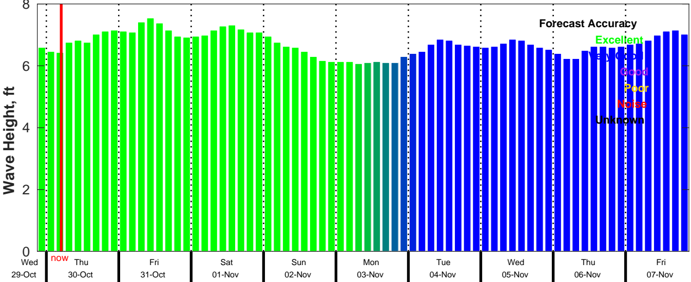
CMEMS Wave Forecast for NDBC 41040 from 29-Oct-2025 21:00:00 to 07-Nov-2025 21:00:00
