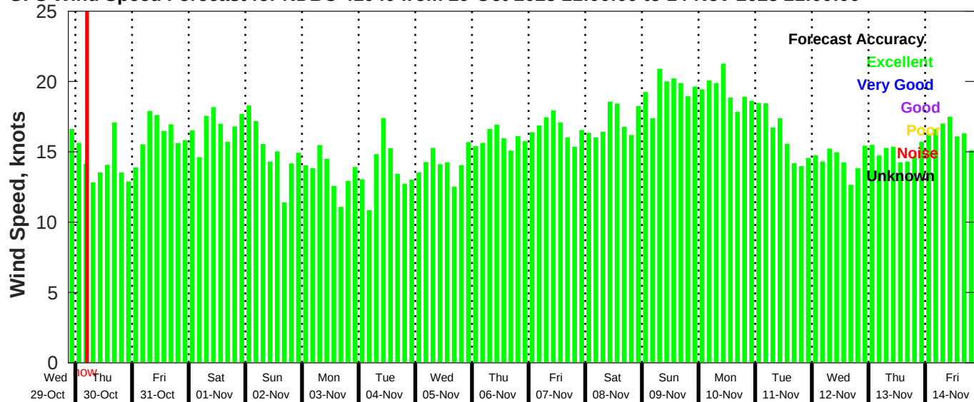
GFS Wind Speed Forecast for NDBC 41040 from 29-Oct-2025 21:00:00 to 14-Nov-2025 21:00:00
