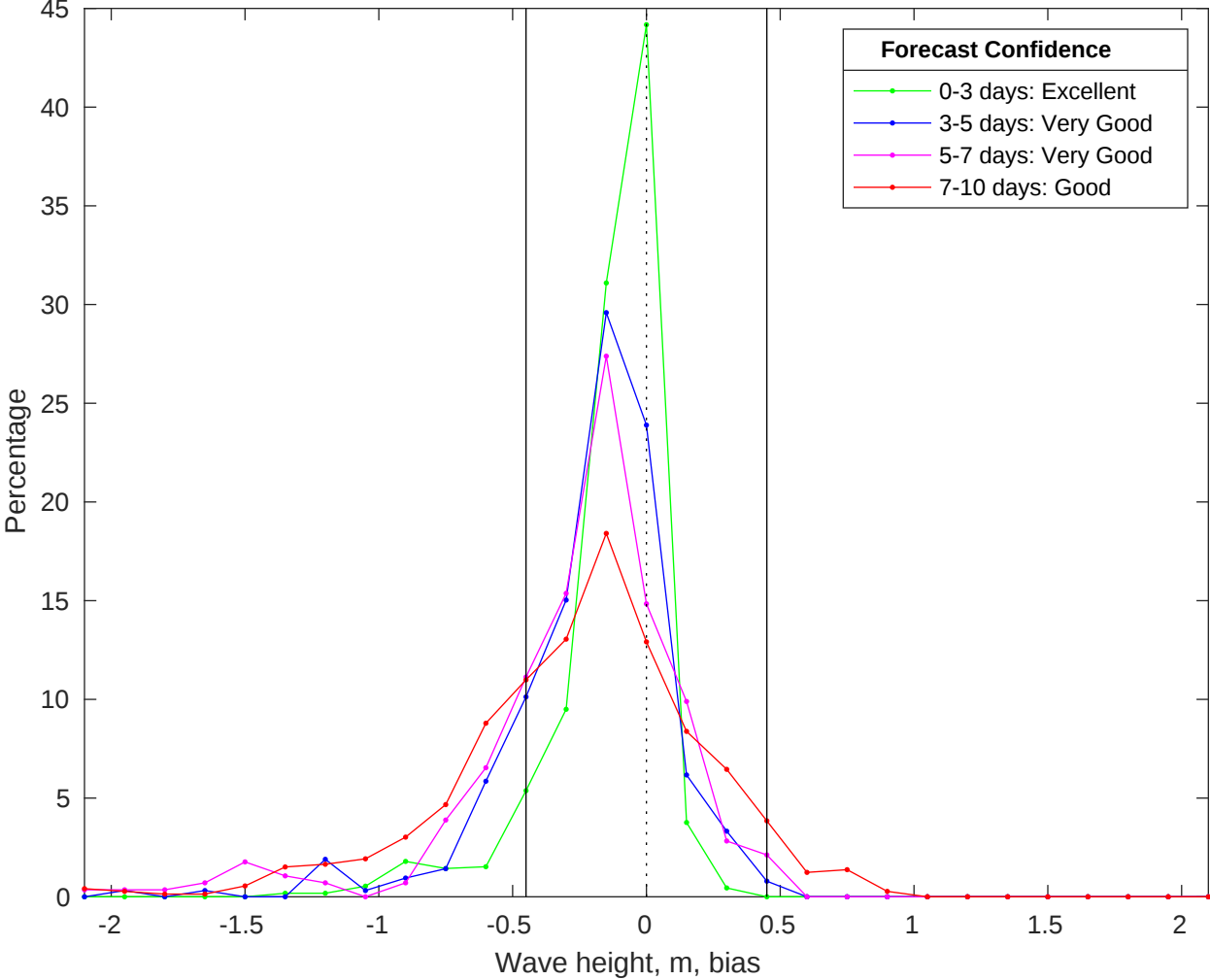
NDBC 42019 vs CMEMS Waves Bias Histogram: 30-Oct-2025
