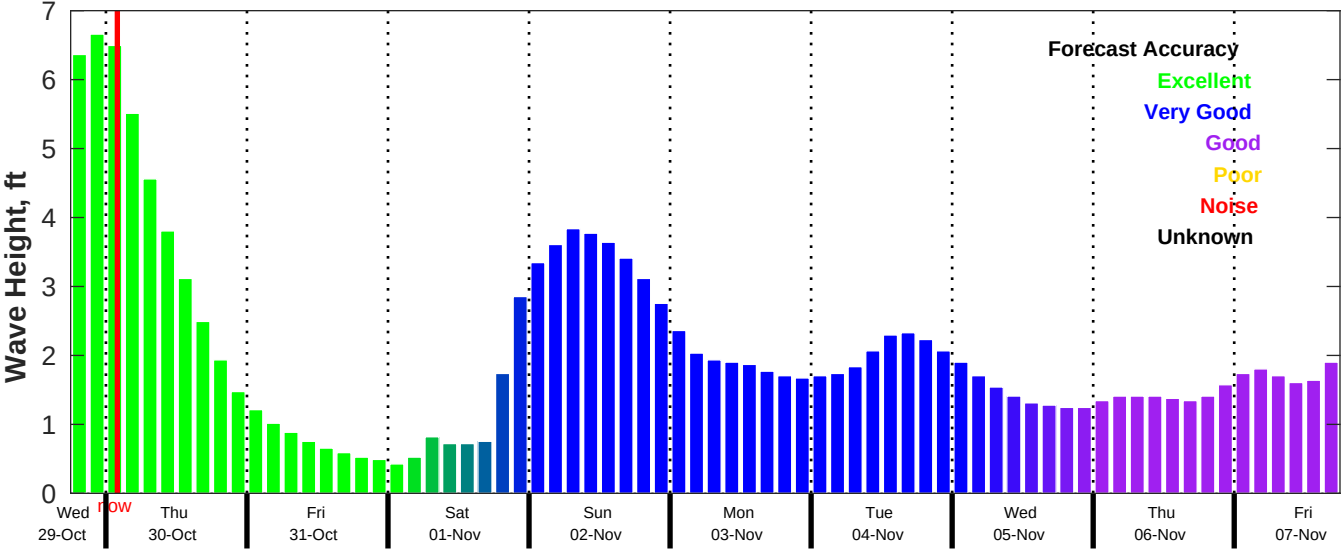
CMEMS Wave Forecast for NDBC 42019 from 29-Oct-2025 18:00:00 to 07-Nov-2025 18:00:00
