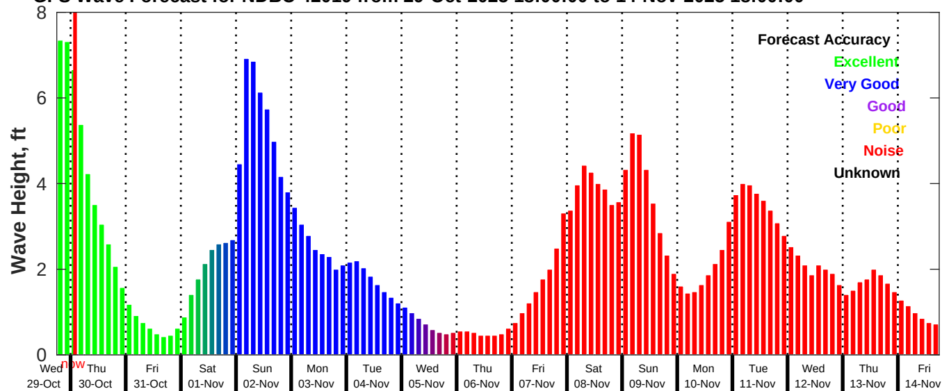
GFS Wave Forecast for NDBC 42019 from 29-Oct-2025 18:00:00 to 14-Nov-2025 18:00:00
