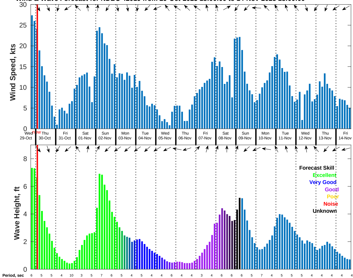
Wind & Wave Forecast for NDBC 42019 from 29-Oct-2025 18:00:00 to 14-Nov-2025 18:00:00
