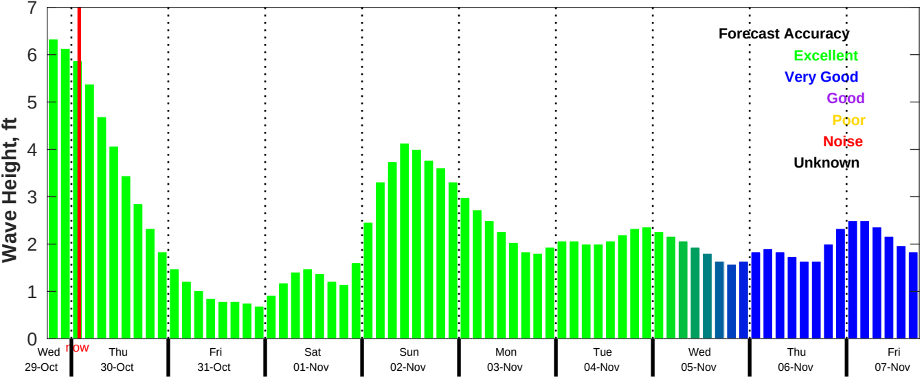
CMEMS Wave Forecast for NDBC 42020 from 29-Oct-2025 18:00:00 to 07-Nov-2025 18:00:00
