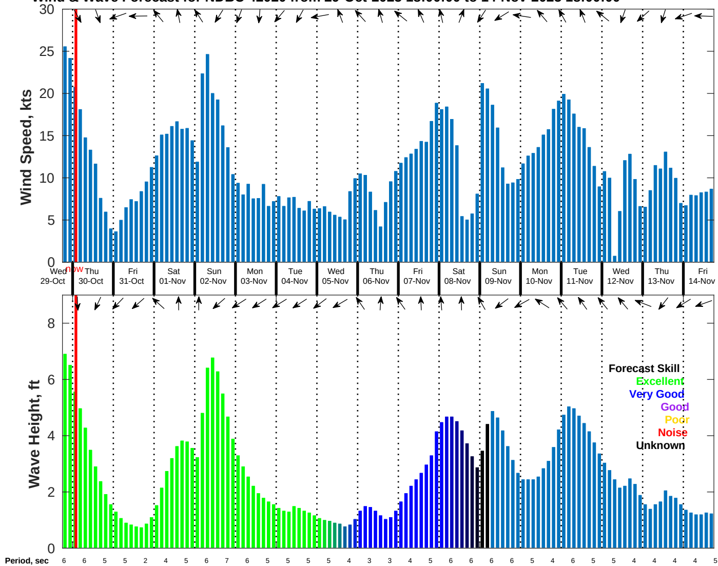
Wind & Wave Forecast for NDBC 42020 from 29-Oct-2025 18:00:00 to 14-Nov-2025 18:00:00
